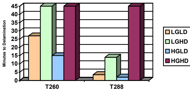
Figure 8 – Time to Delamination Comparisons for 4-7628 Laminate Construction
